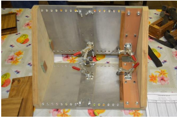
Aluminium jig developed and made by Leon Wolmarans for the safe jointing of wooden boxes.
